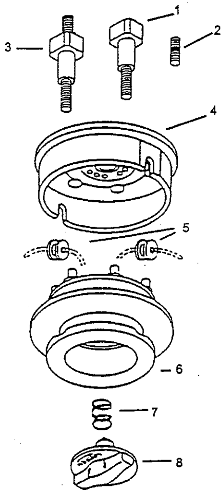
840643 & 840645 Manual Feed
