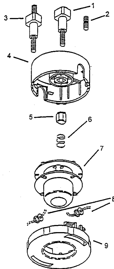
840642 & 840644 Semi-Automatic Feed
